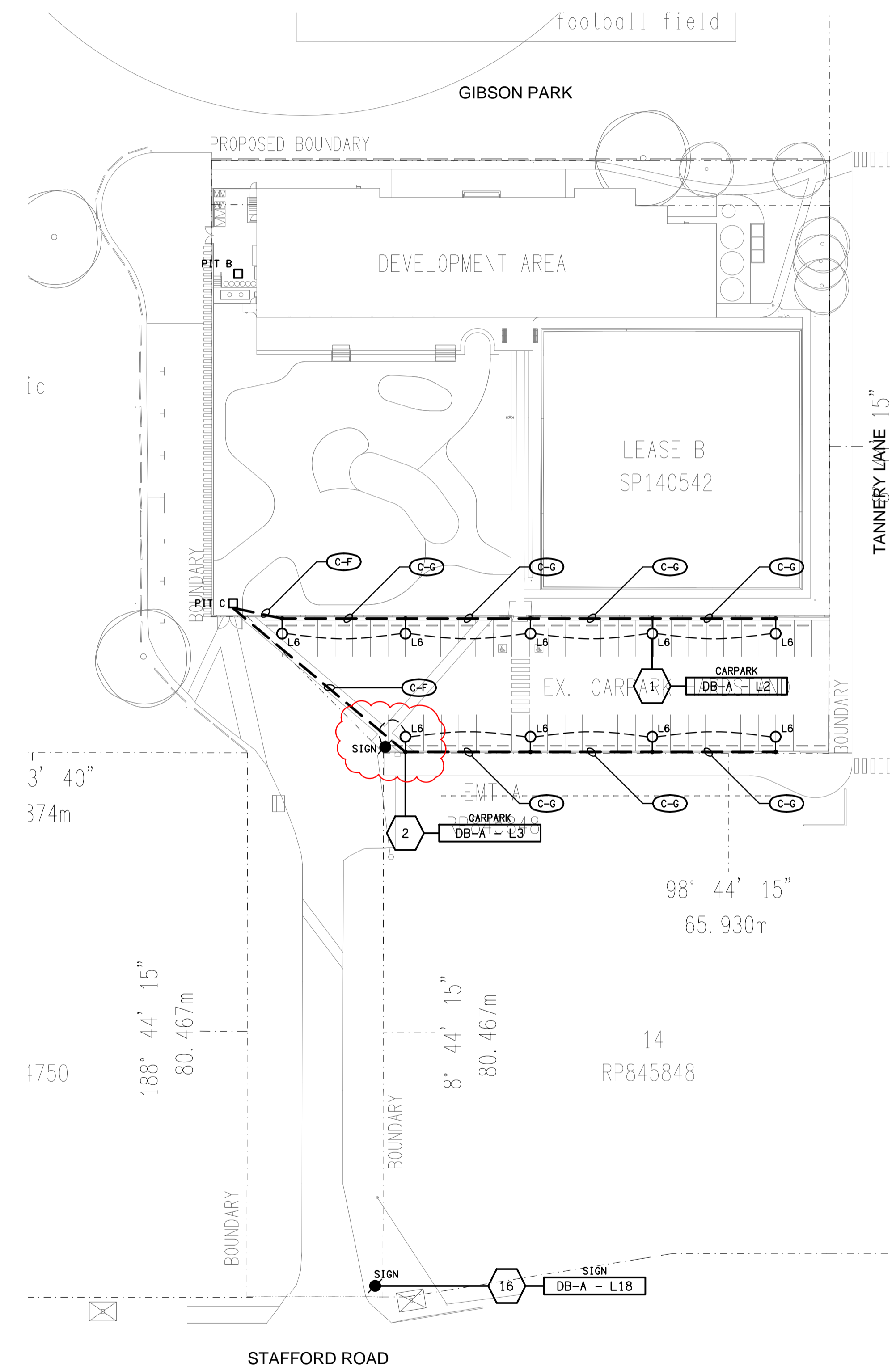
SITE PLAN CARPARK & DRIVEWAY LIGHTING SCALE 1: 500
